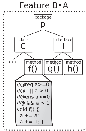
Figure 7: JML handling is transparent to FeatureHouse. JML is parsed after primary FST construction and adds additional granularity to the FST. After superimposition, the additional granularity is deconstructed.
