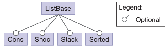
Figure 8: Feature model of the product line ListPL
