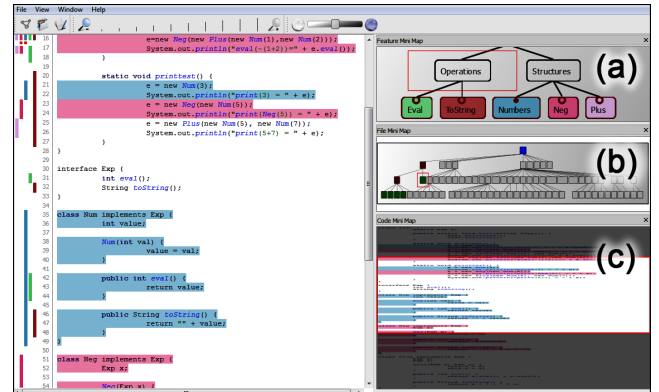
Figure 1: Screenshot of View Infinity . The user interface consists of two parts, left: zoomable main view (currently zoomed to code view), right: mini maps for giving contextual information and showing the visited model layers, feature mini map (a), file mini map (b), code mini map (c). Red rectangles indicate currently focused items.
