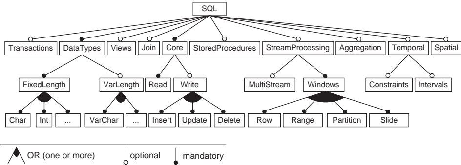
Figure 2: Feature diagram for a subset of SQL that supports core functionality and several extensions.
