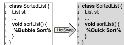
Figure 2: Class schema keeping changes.
