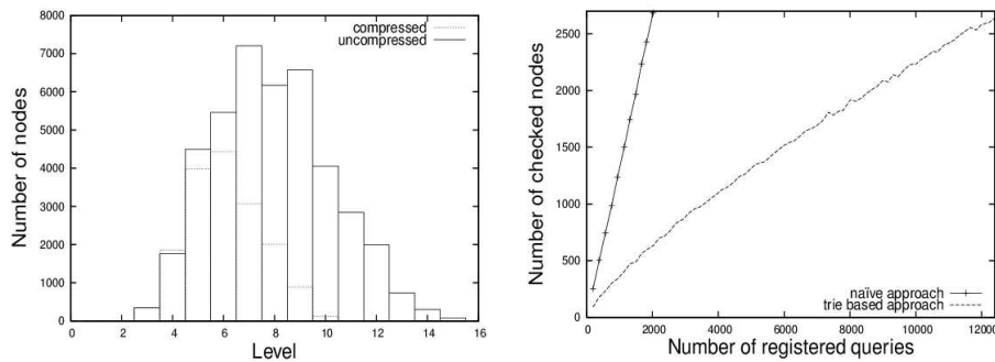
(a) Number of trie-nodes per trie-level (15,000 queries; 12,766 different queries)
