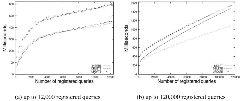
Fig. 4. Correlation between duration of updates and number of registered queries
