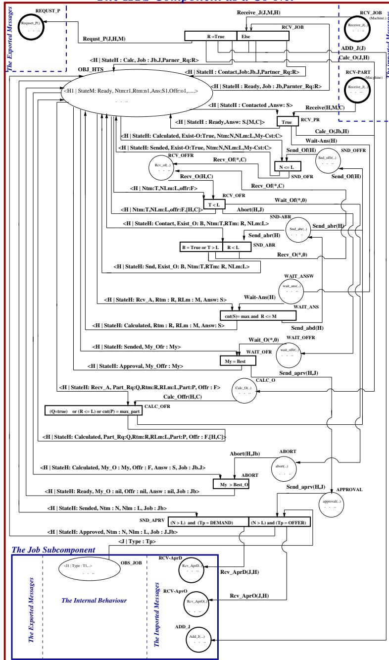
Fig. 3. The HTS CO-NETS Specification.
