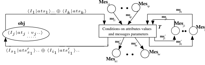
Fig. 2. The Intra-Component Computation Pattern.
