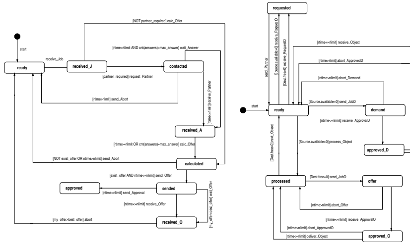
Fig. 1. State Diagram of HTS and Machine Classes
