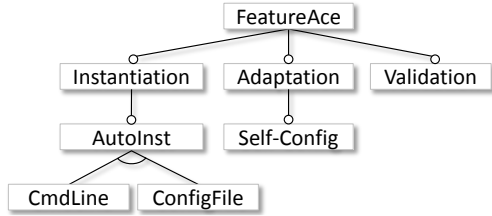
Figure 6. The feature model of FeatureAce. Customization of dynamic product instantiation and runtime adaptation capabilities is achieved by selecting the corresponding features.
